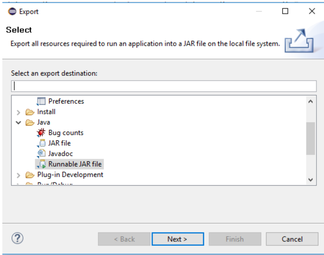
Figure 46. Export wizard
