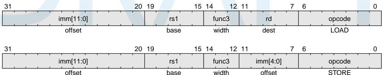
Figure 13. Load and store instructions
