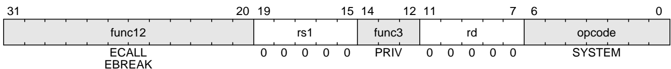
Figure 15. Environment call and breakpoint instructions
