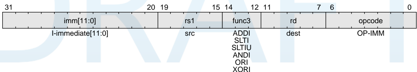
Figure 5. Integer Computational Instructions
