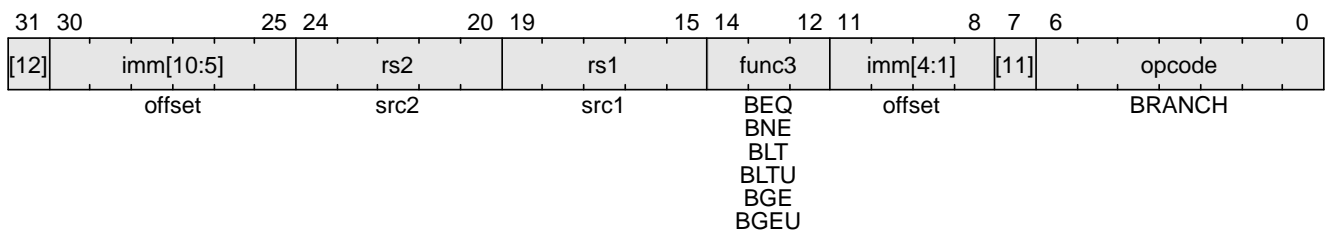
Figure 12. Conditional branches
