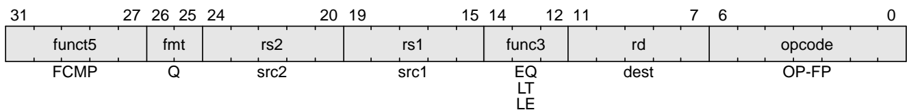
Figure 52. Quad-precision floating-point compare
