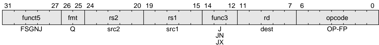
Figure 51. Quad-precision convert and move interchangeably XQ-QX
