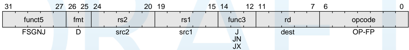
Figure 43. Double-precision sign-injection
