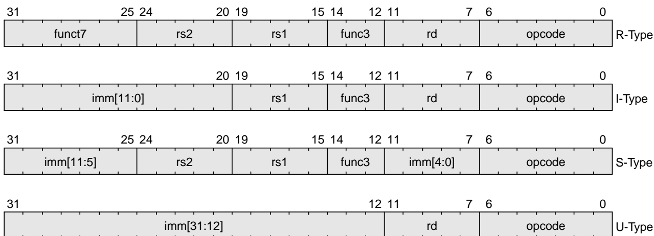
Figure 2. RISC-V base instruction formats
