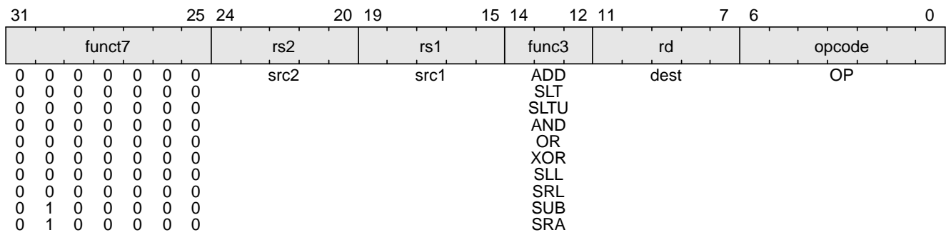
Figure 8. Integer register-register
