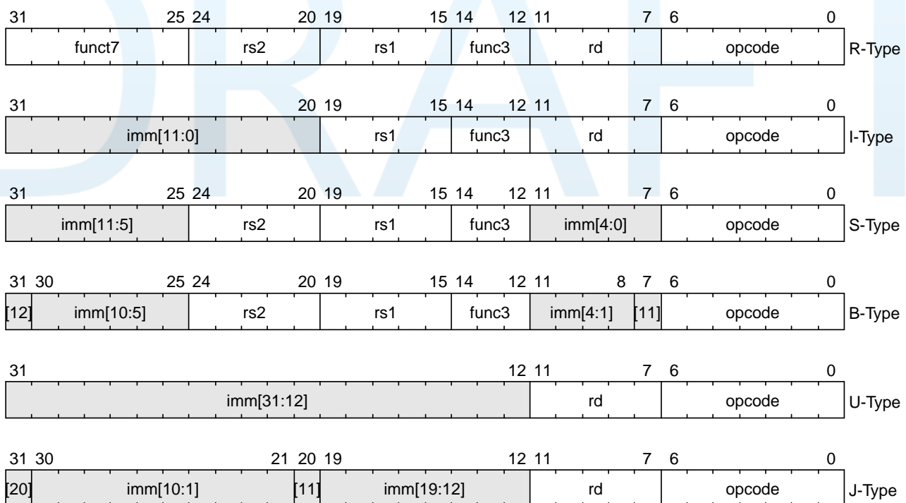
Figure 3. RISC-V base instruction formats.
