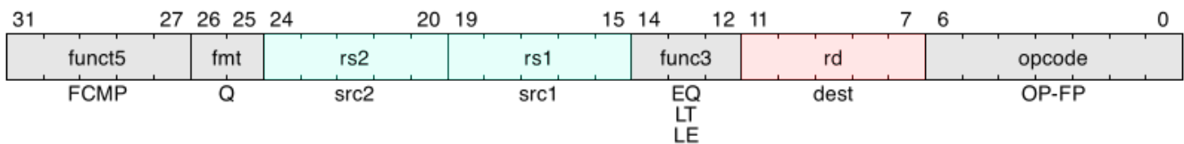
Figure 49. Quad-precision floating-point compare
