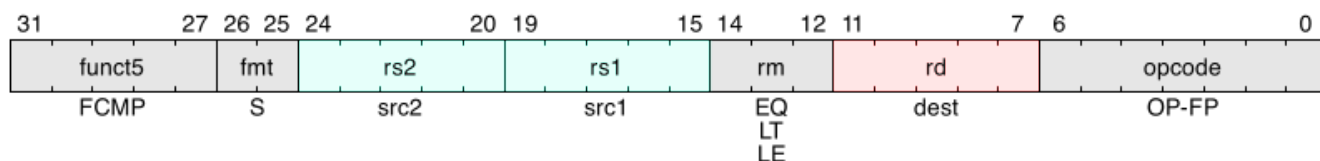
Figure 34. SP floating point compare
