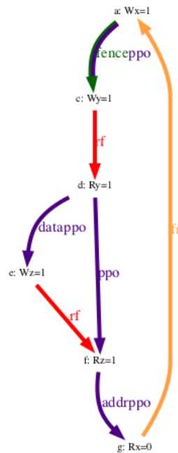
Figure 62. Because of PPO rule 12 and the data dependency from (d) to (e), (d) must also precede (f) in the global memory order (outcome forbidden)
