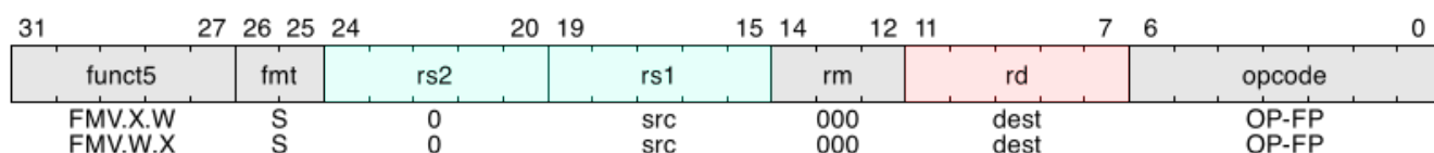
Figure 33. SP floating point move
