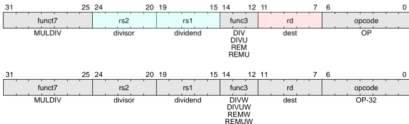
Figure 23. Division operation instructions
