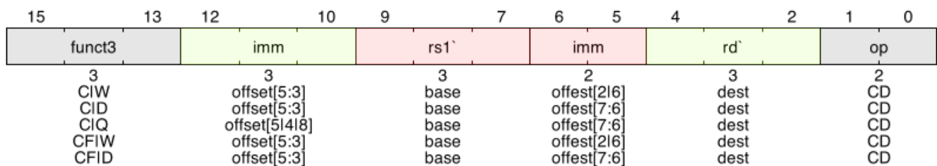
Figure 53. Compressed, register-based load and stores
