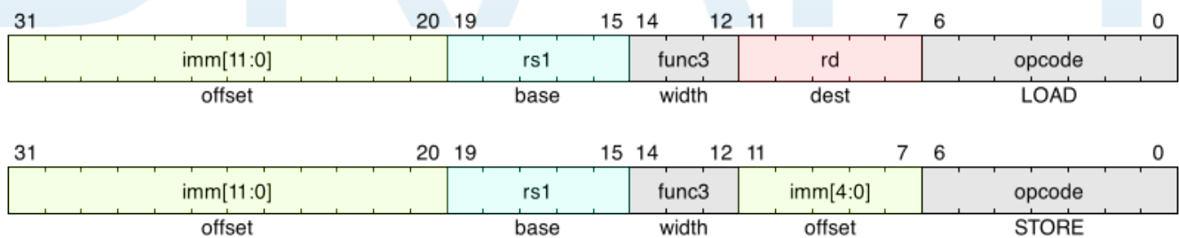
Figure 21. Load and store instructions
