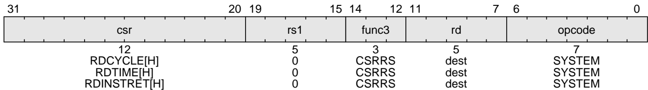
Figure 27. Base counters and timers
