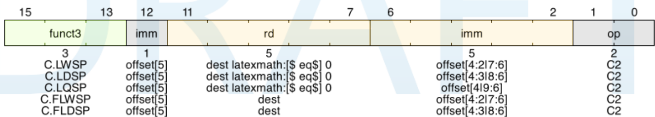
Figure 51. Stack-Pointer-Based Loads and Stores
