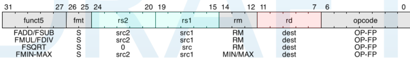
Figure 30. Single-Precision Floating-Point Computational Instructions
