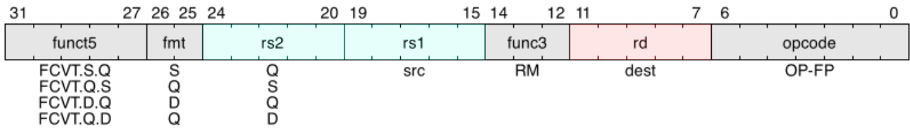
Figure 47. Quad-precision convert and move interchangeably
