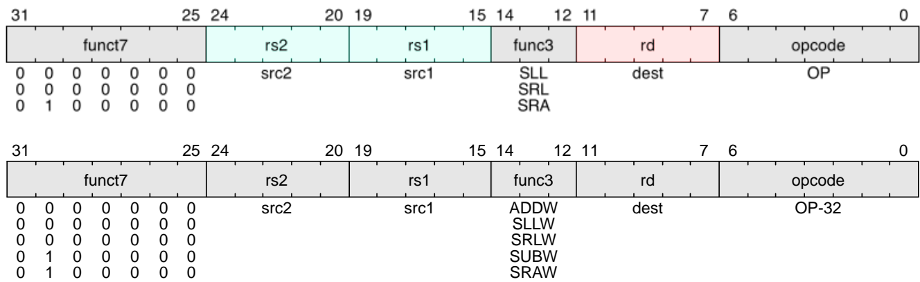
Figure 20. RV64I integer register-register instructions
