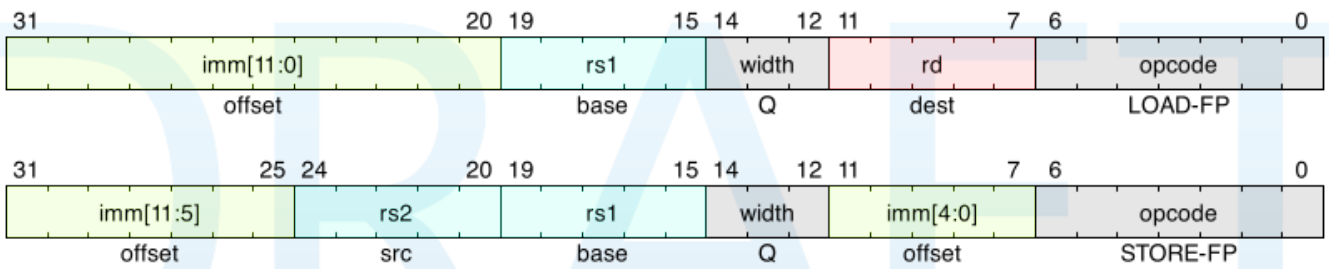
Figure 44. Quad-precision load and store
