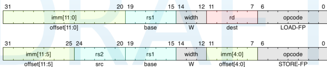
Figure 29. SP load and store
