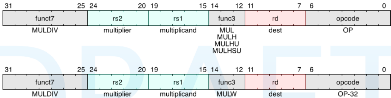
Figure 22. Multiplication operation instructions
