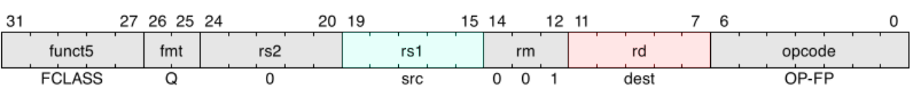
Figure 50. Quad-precision floating point classify
