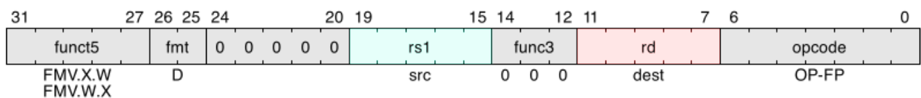
Figure 41. Double-precision float move to rd
