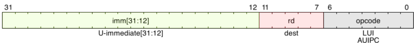
Figure 6. Integer register-immediate, U-immediate
