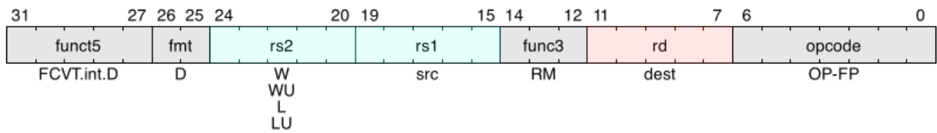
Figure 38. Double-precision float convert and move
