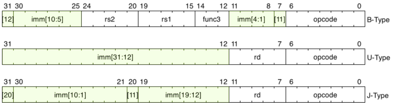
Figure 2. RISC-V base instruction formats.
