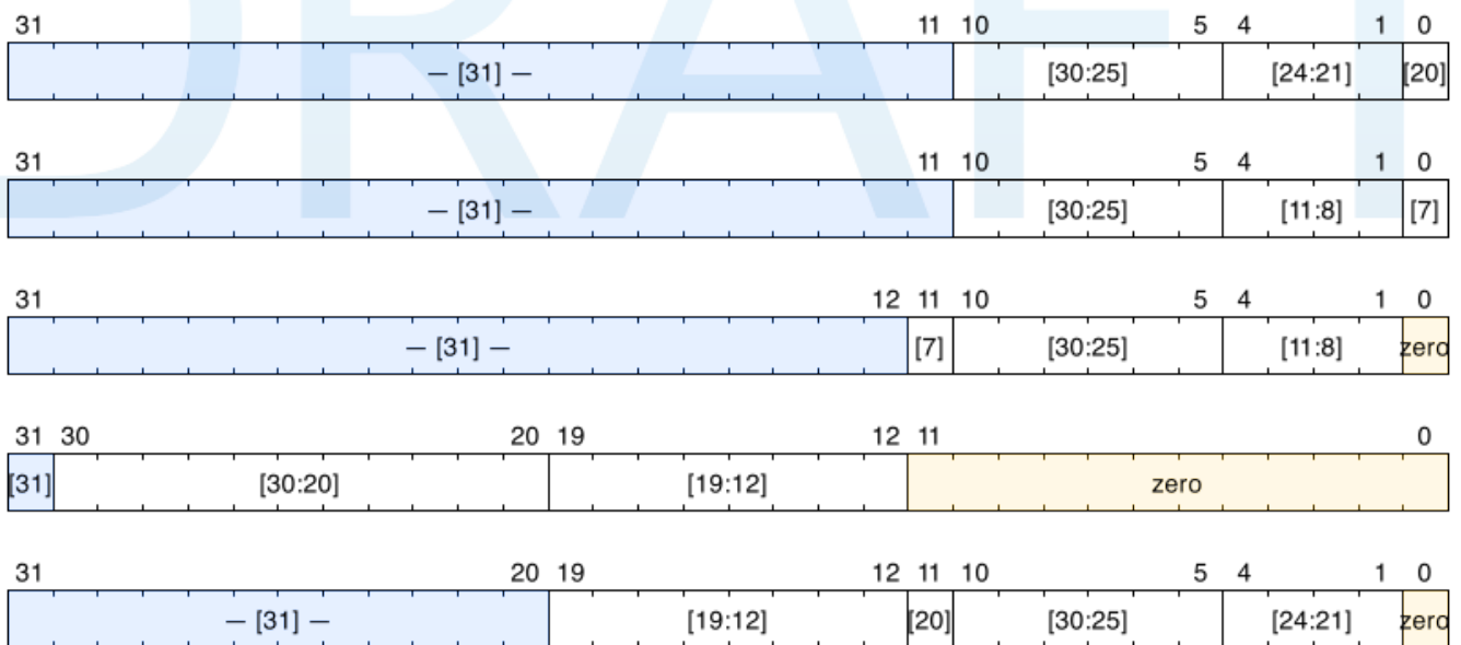
Figure 3. Immediate variants for I, S, B, U, and J
