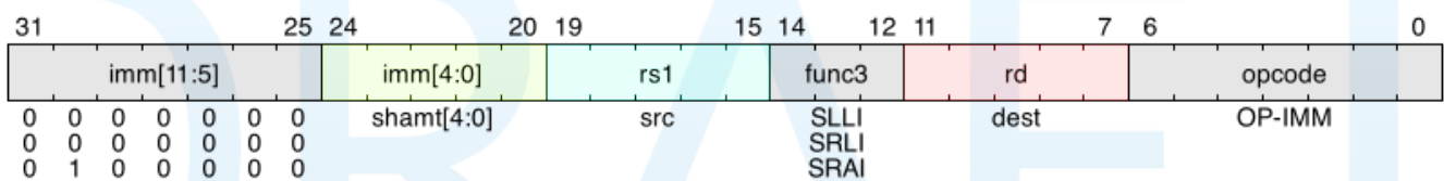
Figure 5. Integer register-immediate, SLLI, SRLI, SRAI
