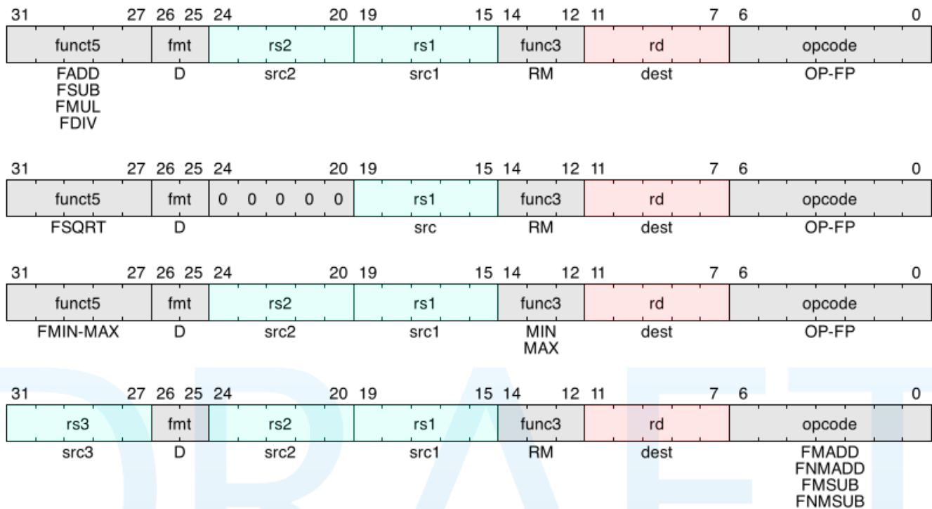
Figure 37. Double-precision float computational
