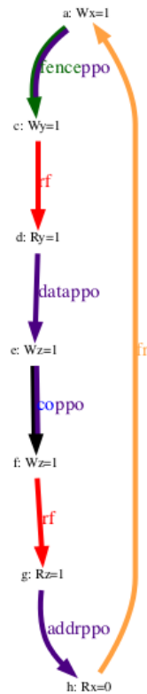
Figure 63. Because of the extra store between (e) and (g), (d) no longer necessarily precedes (g) (outcome permitted)
