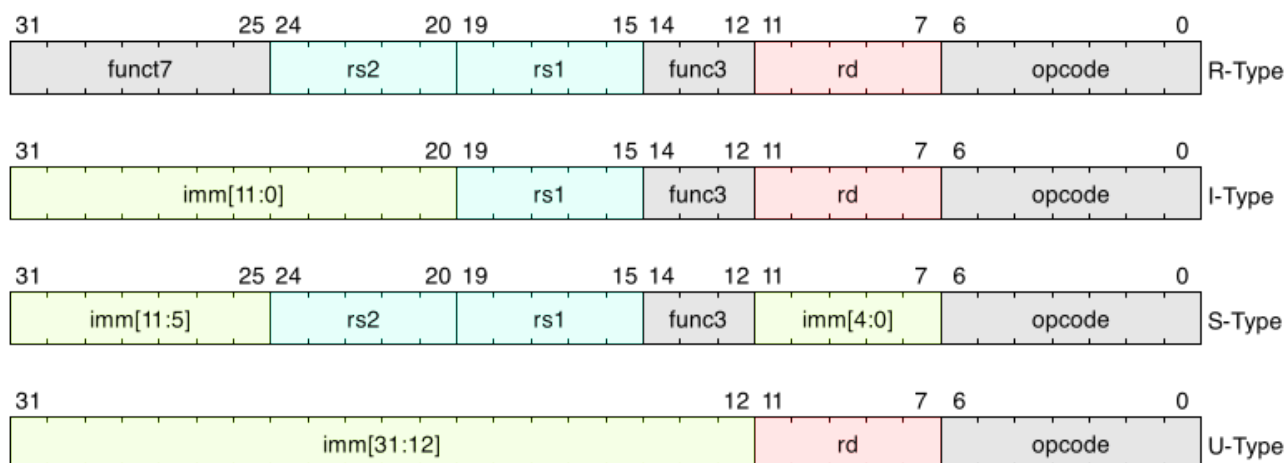
Figure 1. RISC-V base instruction formats
