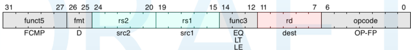
Figure 42. Double-precision float compare
