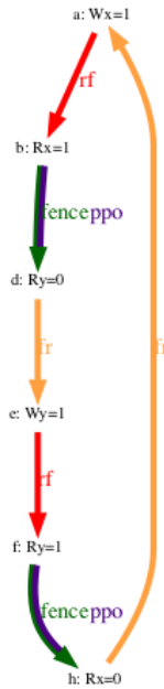
Figure 57. A store buffer forwarding litmus test (outcome permitted)
