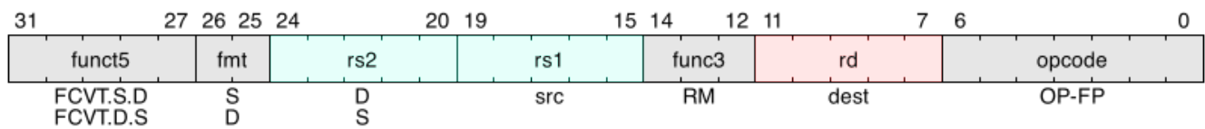
Figure 39. Double-precision FCVT.S.D and FCVT.D.S
