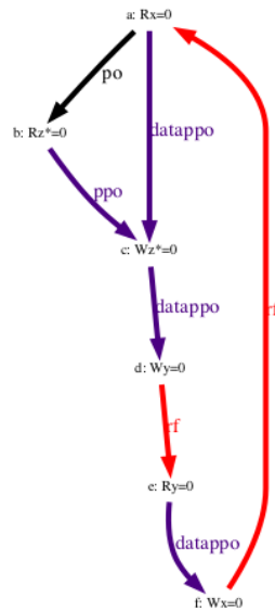
Figure 61. A variant of the LB litmus test (outcome forbidden)
