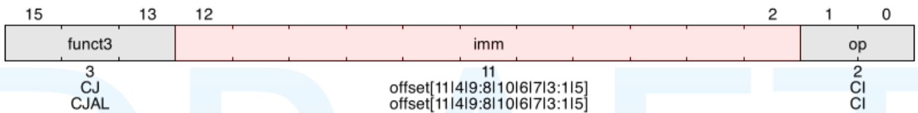
Figure 55. Compressed, CJ format load and store
