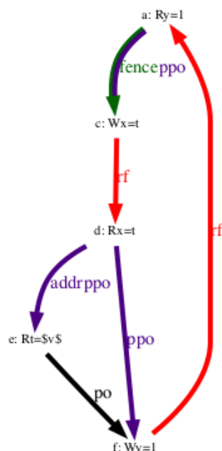
Figure 64. Because of the address dependency from (d) to (e), (d) also precedes (f) (outcome forbidden)
