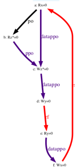
Figure 59. A sample litmus test and one forbidden execution ( aO=1 )
