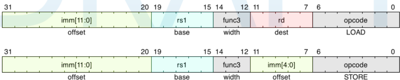
Figure 12. Load and store instructions
