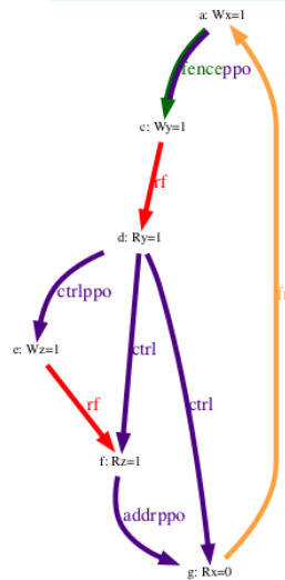
Figure 58. The “PPOCA” store buffer forwarding litmus test (outcome permitted)
