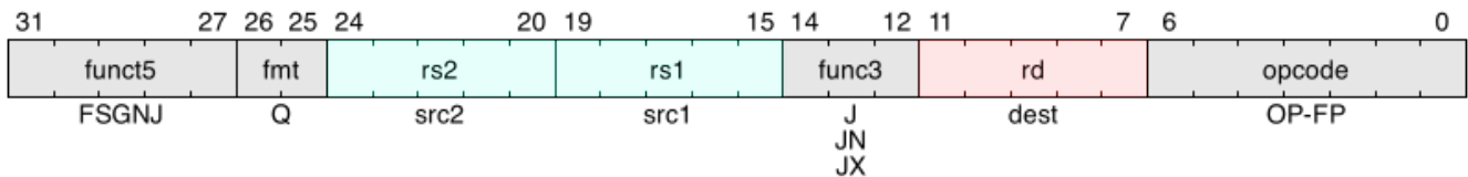
Figure 48. Quad-precision convert and move interchangeably XQ-QX
