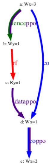
Figure 65. Write subsumption litmus test, allowed execution
