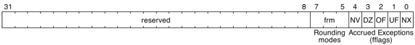
Figure 28. Floating-point control and status register
