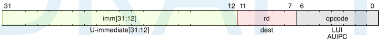
Figure 19. RV64I register-immediate (descr) instructions
