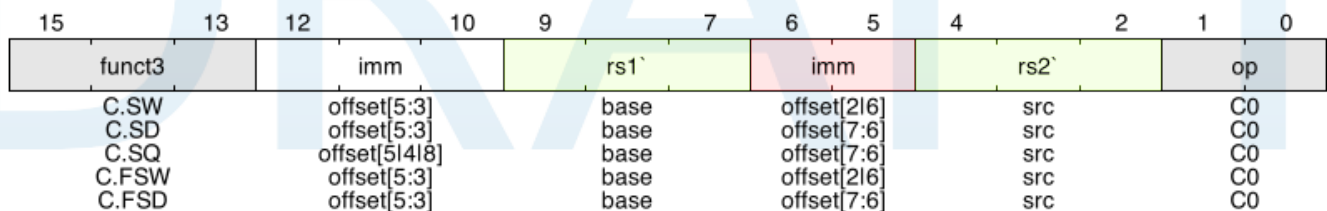
Figure 54. Compressed, CS format load and store
