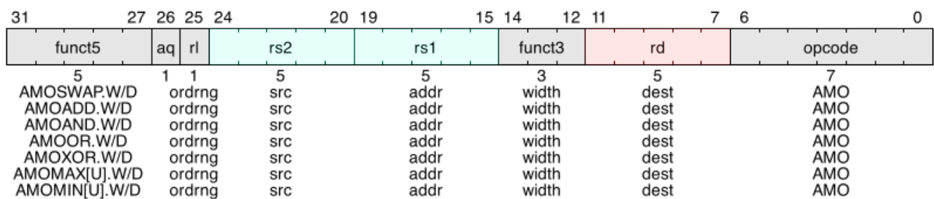
Figure 25. Atomic memory operations
