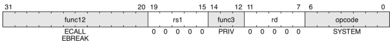
Figure 14. Environment call and breakpoint instructions
