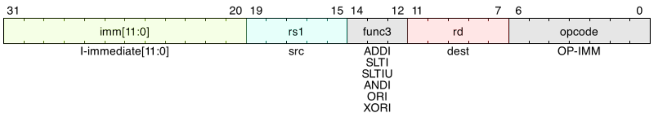
Figure 4. Integer Computational Instructions
