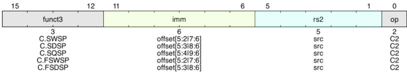
Figure 52. Stack-Pointer-Based Loads and Stores, CSS format
