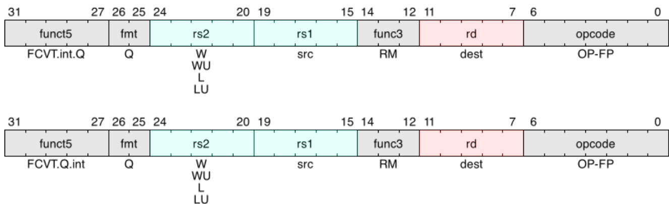
Figure 46. Quad-precision convert and move
