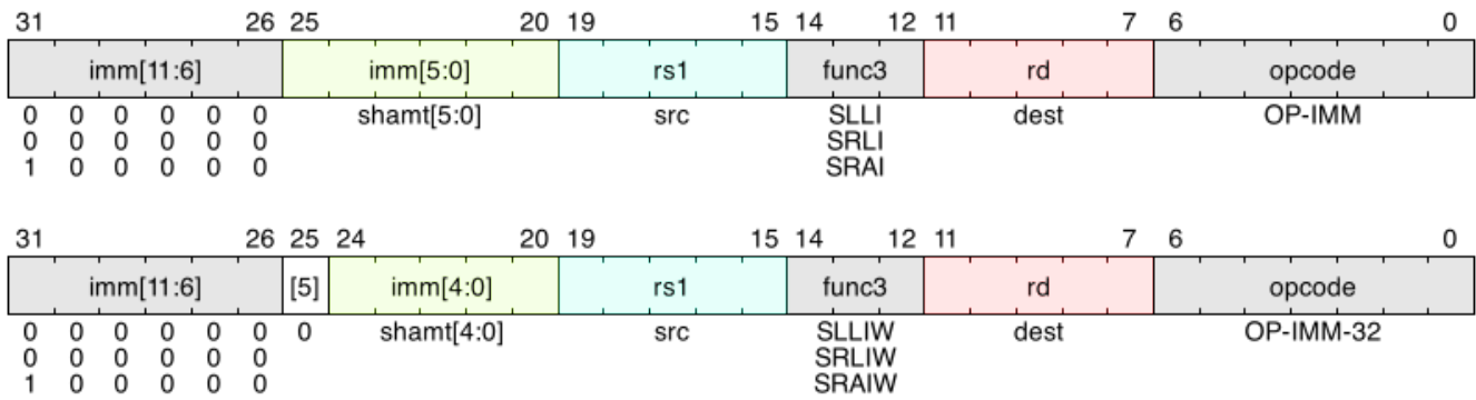
Figure 18. RV64I register-immediate (descr ADDIW) instructions
