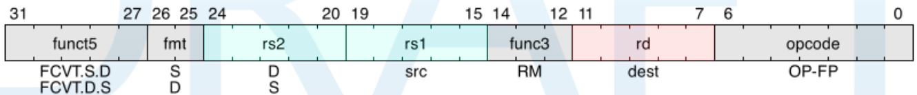
Figure 32. SP float convert and move
