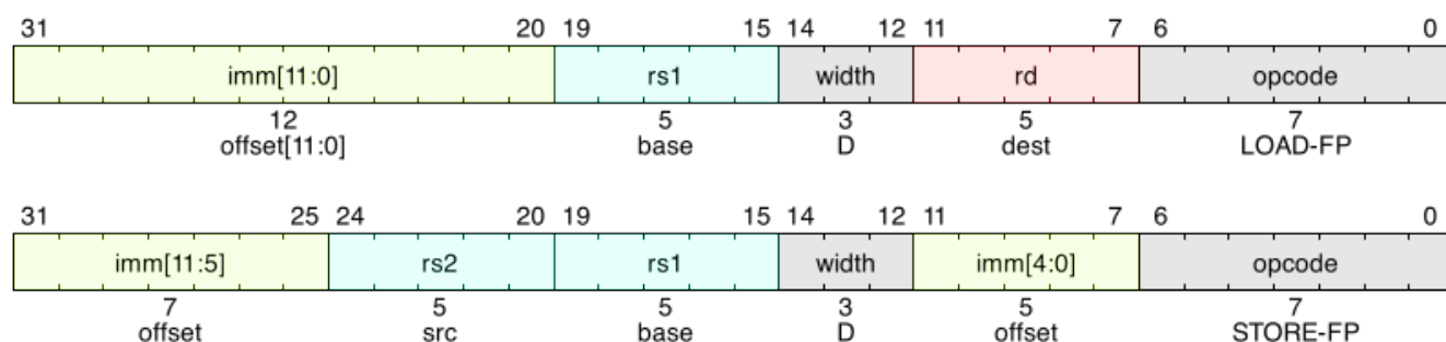
Figure 36. Double-precision load and store
