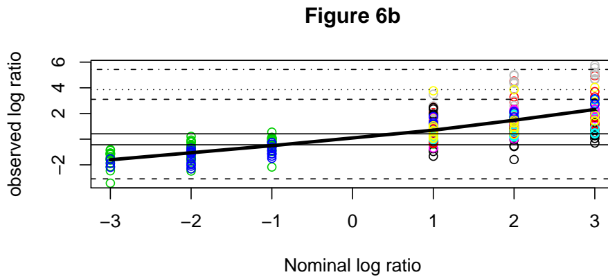
Figure 6: a) Observed log fold changes plotted against nominal log fold changes. The dashed lines represent highest, 25th highest, 100th highest, 25th percentile, 75th percentile, smallest 100th, smallest 25th, and smallest log fold change for the genes that were not differentially expressed. b) Like a) but the observed fold changes were calculated for spiked in genes with nominal concentrations no higher than 2pM.
